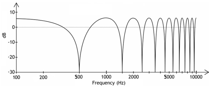
Diagram 5. Example of Comb Filtering
