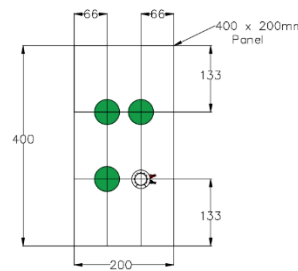
Diagram 3. Ideal Mount Locations
