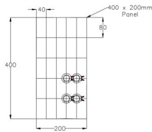
Diagram 7. Mounting Four Exciters
